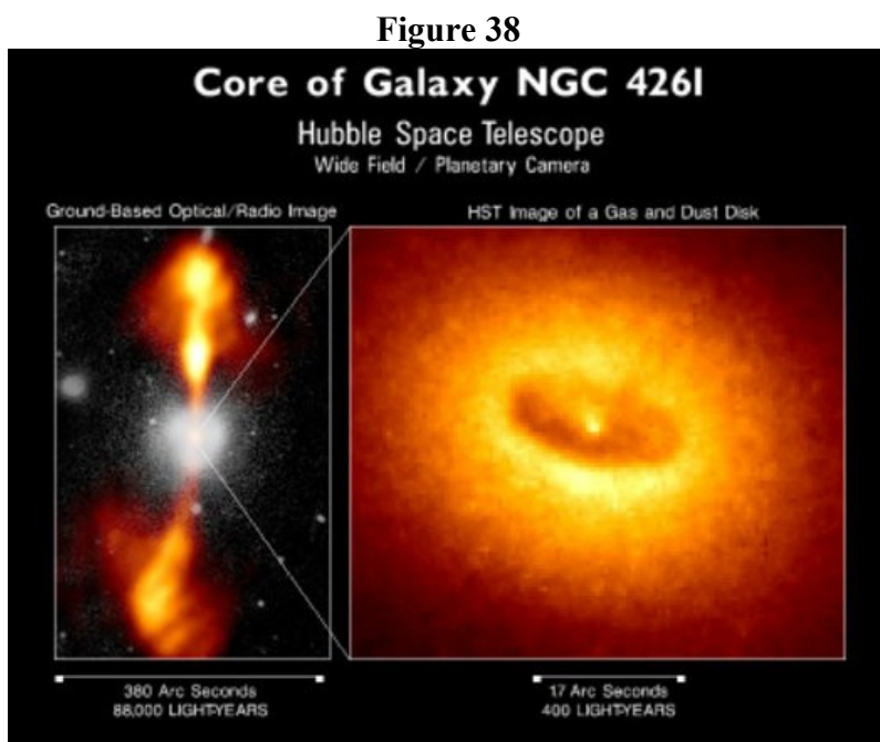
Elliptical Galaxy NGC 4261 [186]
