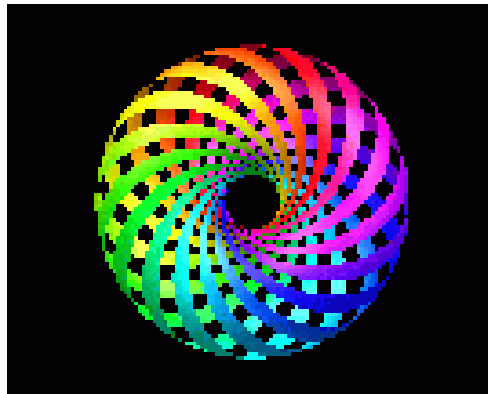
T. Banchoff – Flat Torus in 3-Sphere [ 180 ]
