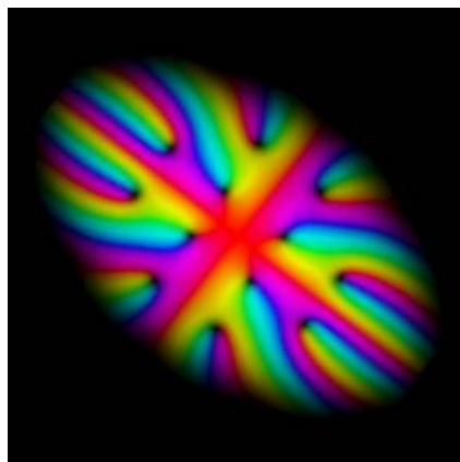
Twelve-vortex array in a rotating Bose-Einstein Condensate
