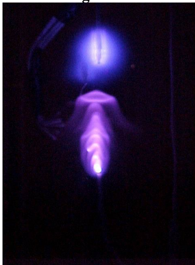
EVO Plasma Discharge [Jin][176]
