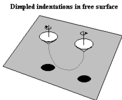
Black Spots Refracted on Pool Floor
