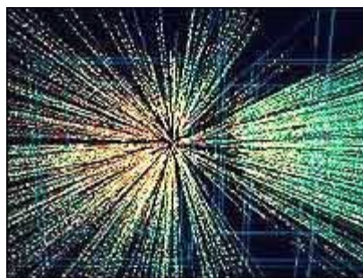
Digital image of Carbon atoms being bombarded by X-rays.
