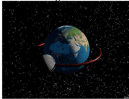
The Earth and Moon interact as a single Soliton
