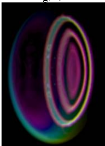
Decay of a Soliton in a Bose-Einstein Condensate Fourth Scale manifestation of condensed mass [image credit NIST]
